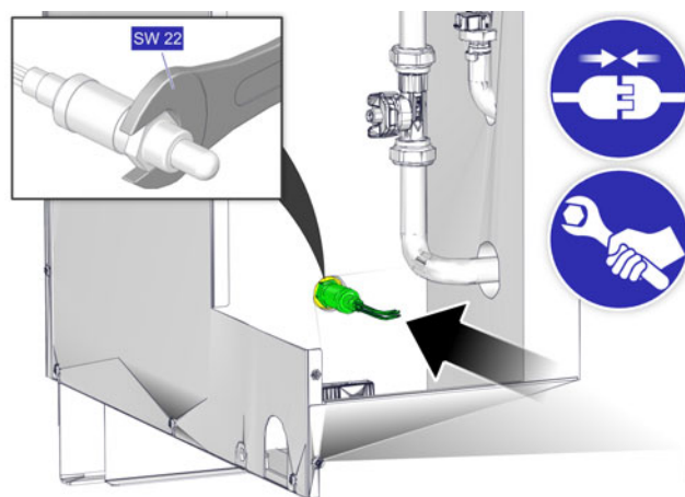
Sl. 10-4: Lambda sonda
