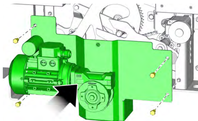
Sl. 8-20: Pogon
