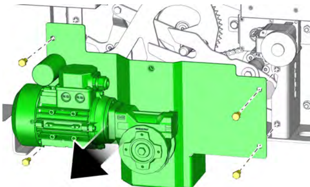
Sl. 8-13: Pogon
