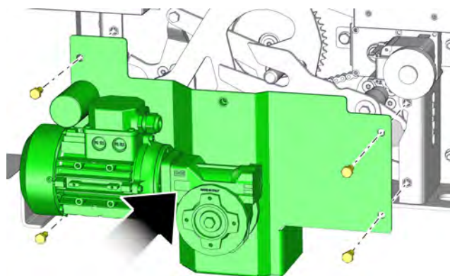
Sl. 8-20: Pogon
